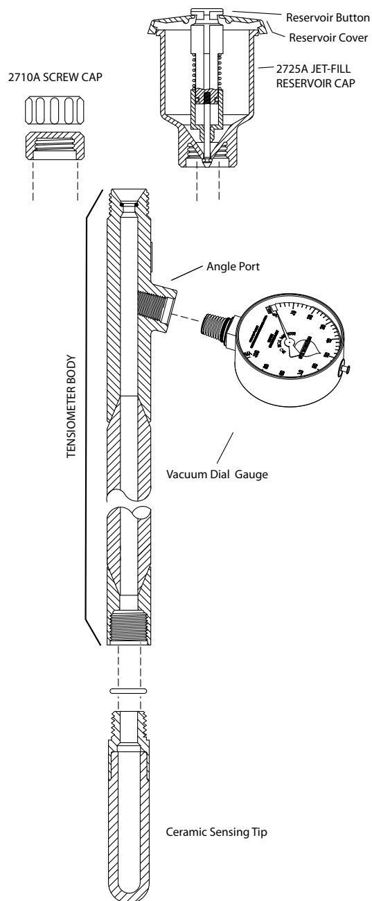
(Fig. 2) 2710A and 2725A Tensiometer Parts
